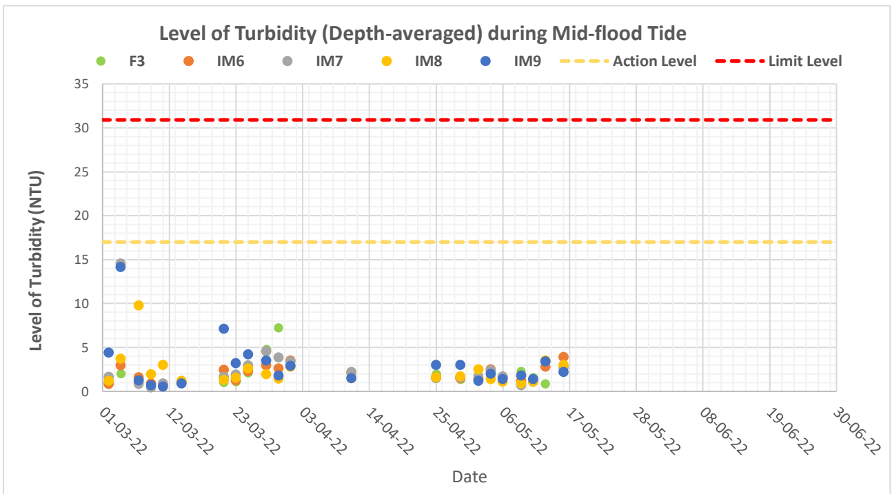
Figure F3c: Levels of Depth-averaged Turbidity (NTU) at control station (F3) and impact stations (IM6-IM9) under Group 3 during mid-flood tides in the past four months (i.e. March 2022 to June 2022)
