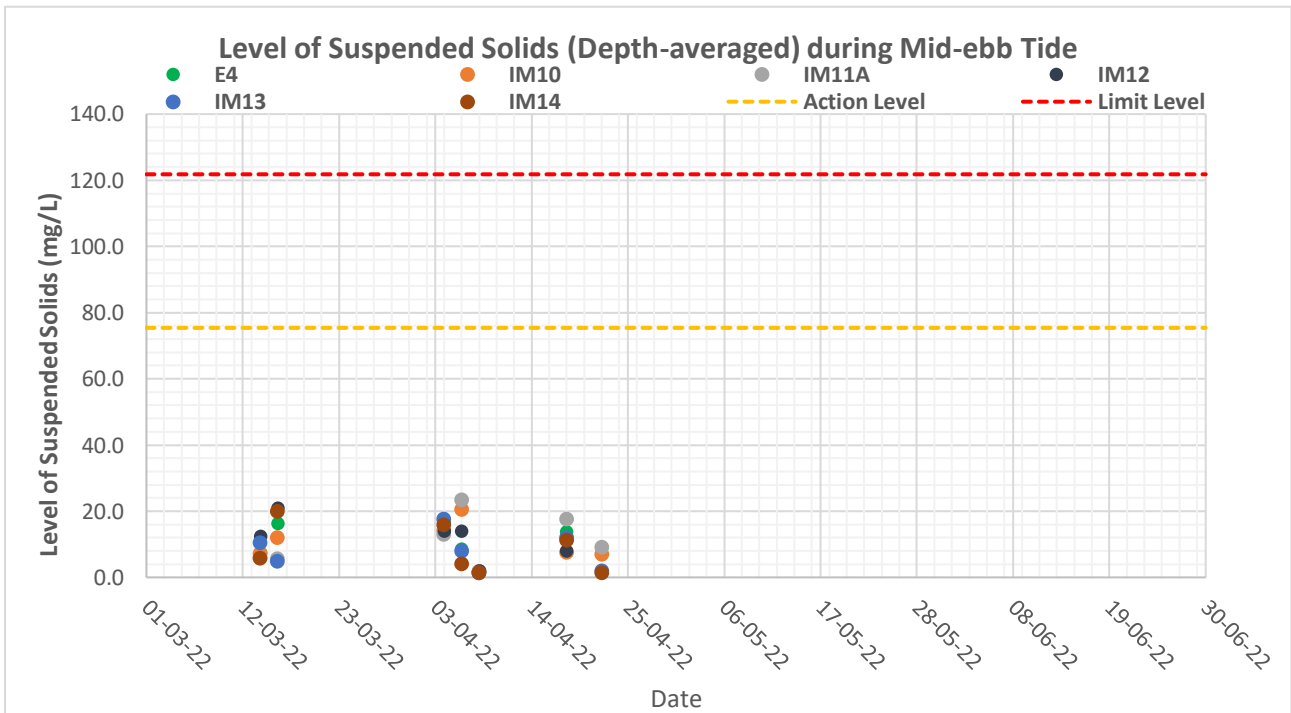
Figure F4b: Levels of Depth-averaged Suspended Solids (mg/L) at control station (E4) and impact stations (IM10-IM14) under Group 4 during mid-ebb tides in the past four months (i.e. March 2022 to June 2022)
