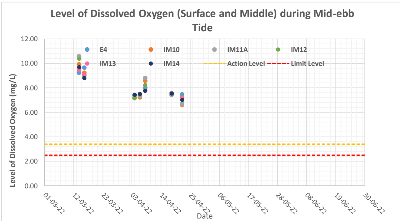
Figure F1b: Levels of Surface and Middle Dissolved Oxygen (mg/L) at control station (E4) and impact stations (IM10-IM14) under Group 4 during mid-ebb tides in the past four months (i.e. March 2022 to June 2022)
