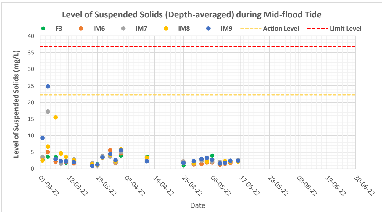
Figure F4c: Levels of Depth-averaged Suspended Solids (mg/L) at control station (F3) and impact stations (IM6-IM9) under Group 3 during mid-flood tides in the past four months (i.e. March 2022 to June 2022)
