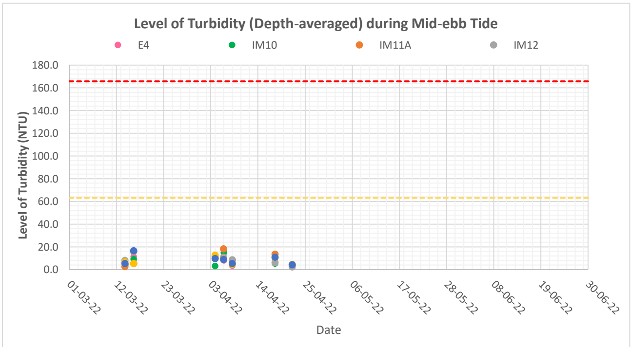
Figure F3b: Levels of Depth-averaged Turbidity (NTU) at control station (E4) and impact stations (IM10-IM14) under Group 4 during mid-ebb tides in the past four months (i.e. March 2022 to June 2022)
