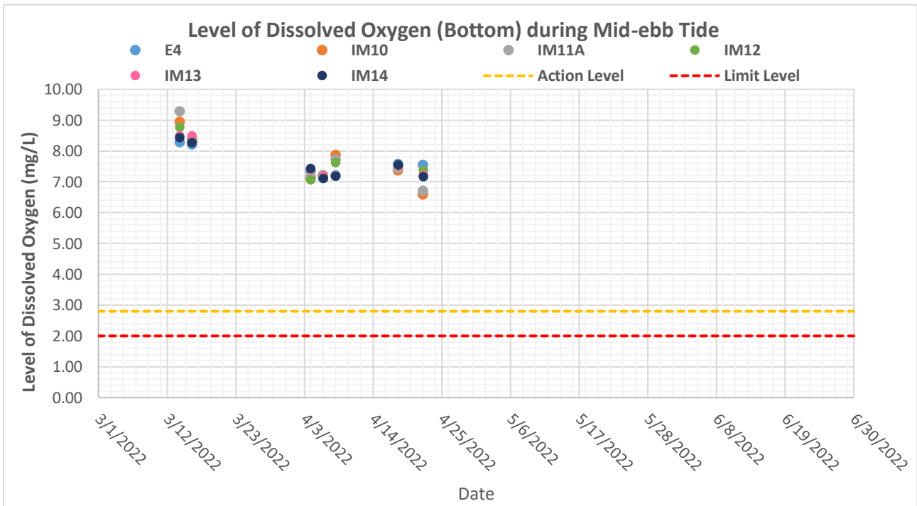
Figure F2b: Levels of Bottom Dissolved Oxygen (mg/L) at control station (E4) and impact stations (IM10-IM14) under Group 4 during mid-ebb tides in the past four months (i.e. March 2022 to June 2022)
