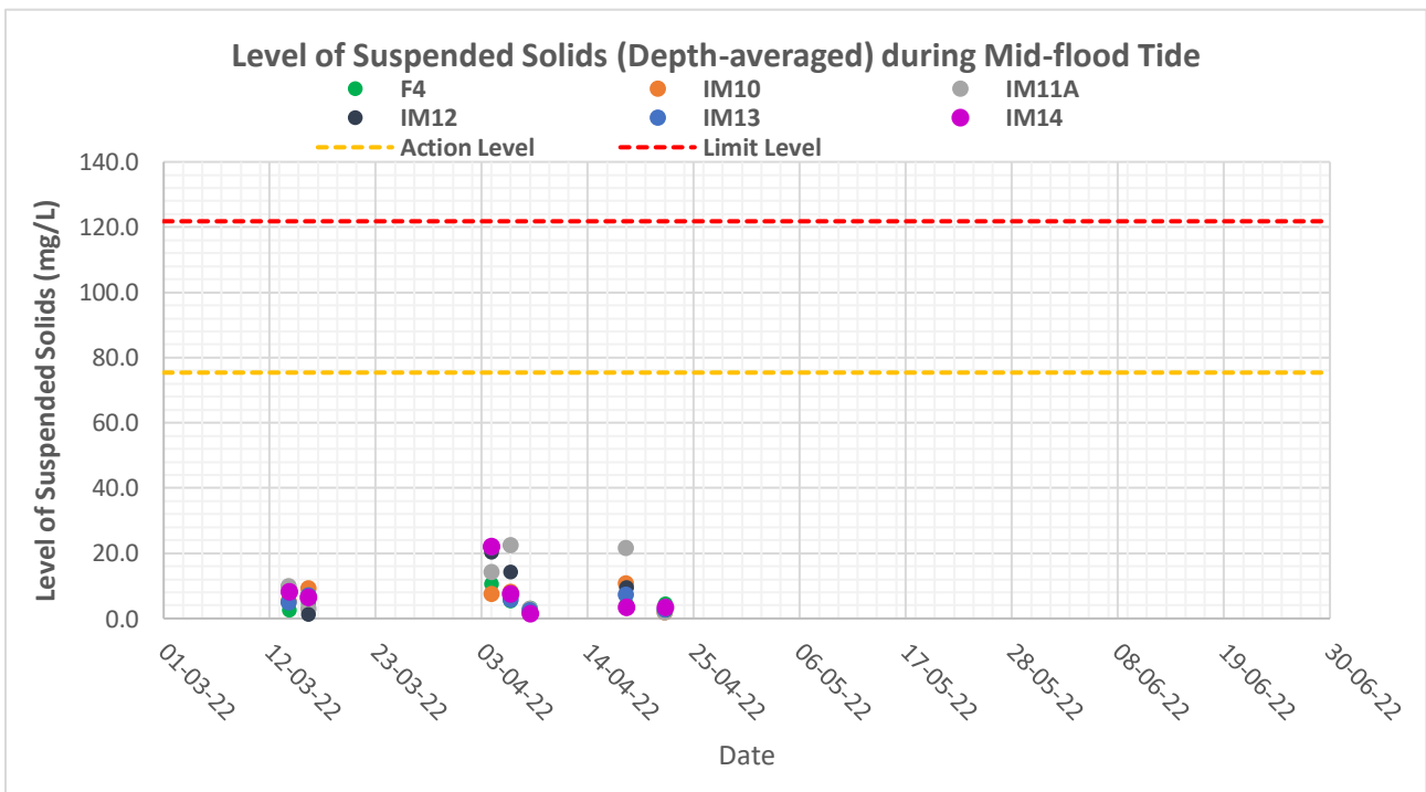
Figure F4d Levels of Depth-averaged Suspended Solids (mg/L) at control station (F4) and impact stations (IM10-IM14) under Group 4 during mid-flood tides in the past four months (i.e. March 2022 to June 2022)
