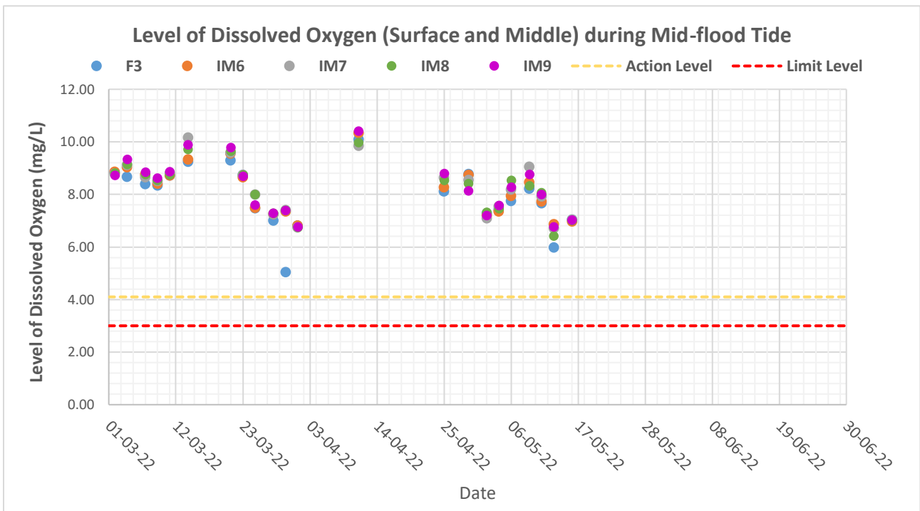
Figure F1c: Levels of Surface and Middle Dissolved Oxygen (mg/L) at control station (F3) and impact stations (IM6-IM9) under Group 3 during mid-flood tides in the past four months (i.e. March 2022 to June 2022)
