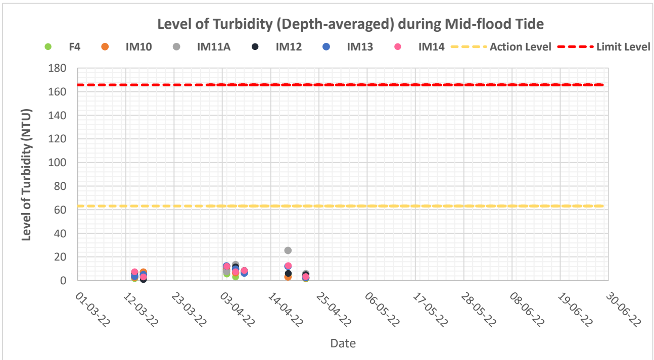
Figure F3d: Levels of Depth-averaged Turbidity (NTU) at control station (F4) and impact stations (IM10-IM14) under Group 4 during mid-flood tides in the past four months (i.e. March 2022 to June 2022)
