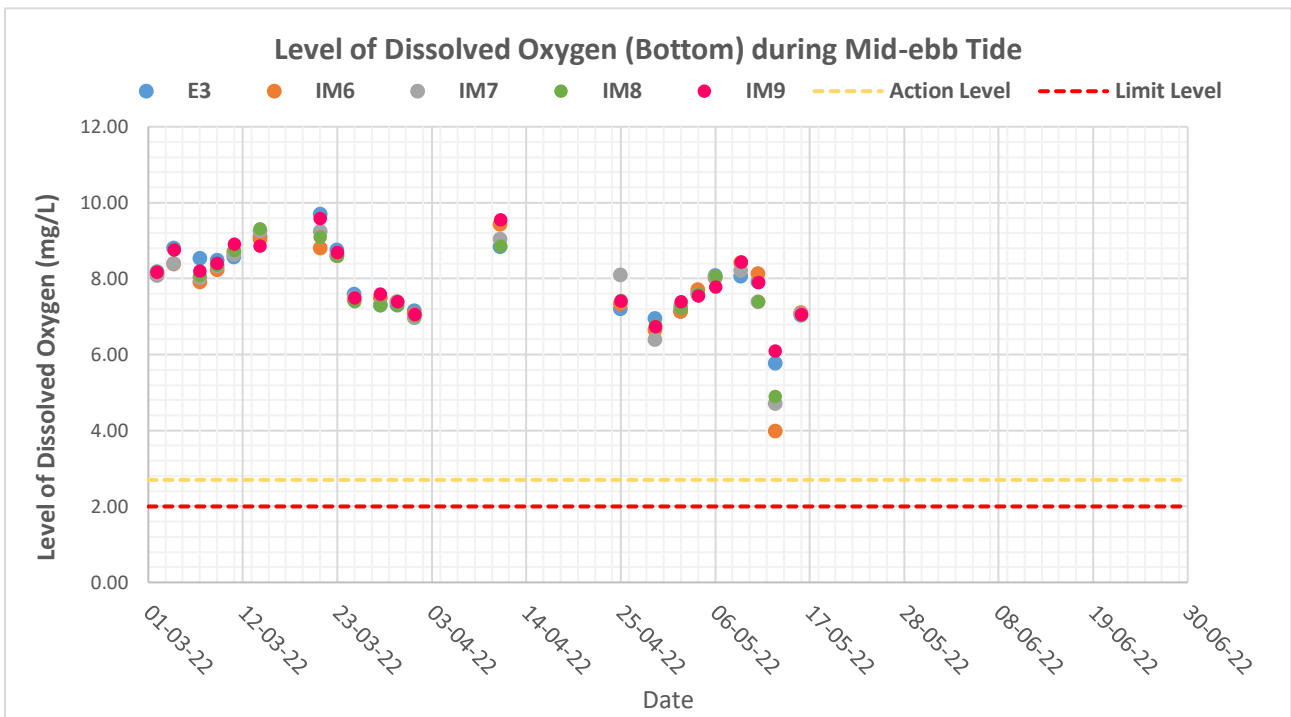
Figure F2a: Levels of Bottom Dissolved Oxygen (mg/L) at control station (E3) and impact stations (IM6-IM9) under Group 3 during mid-ebb tides in the past four months (i.e. March 2022 to June 2022)
