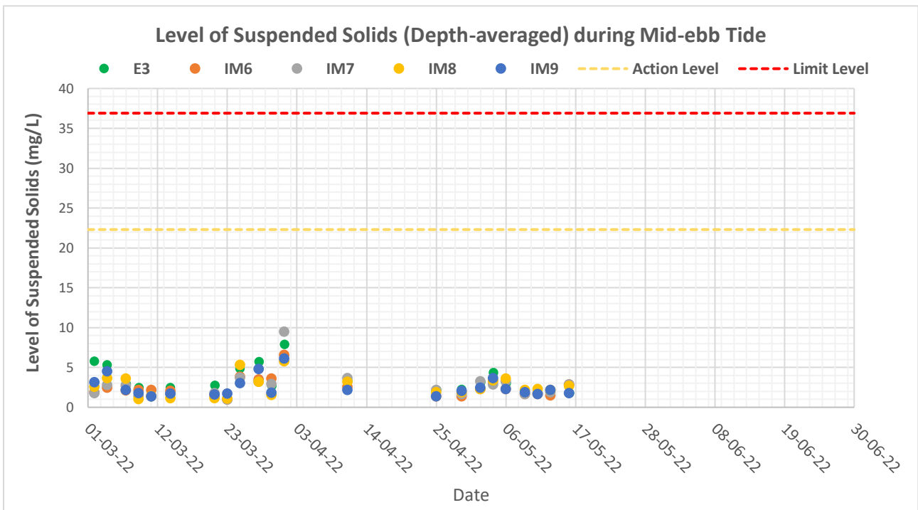
Figure F4a: Levels of Depth-averaged Suspended Solids (mg/L) at control station (E3) and impact stations (IM6-IM9) under Group 3 during mid-ebb tides in the past four months (i.e. March 2022 to June 2022)
