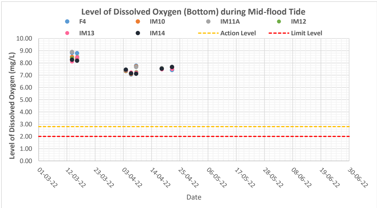
Figure F2d: Levels of Bottom Dissolved Oxygen (mg/L) at control station (F4) and impact stations (IM10-IM14) under Group 4 during mid-flood tides in the past four months (i.e. March 2022 to June 2022)
