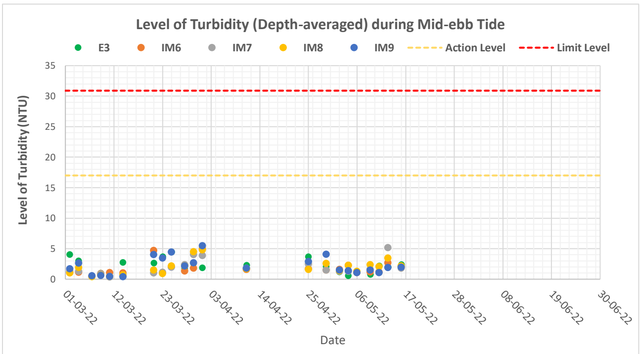
Figure F3a: Levels of Depth-averaged Turbidity (NTU) at control station (E3) and impact stations (IM6-IM9) under Group 3 during mid-ebb tides in the past four months (i.e. March 2022 to June 2022)
